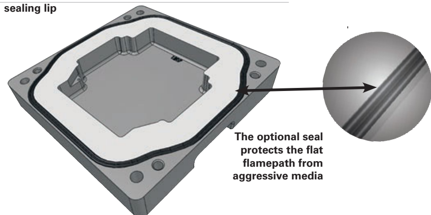
sealing lip
